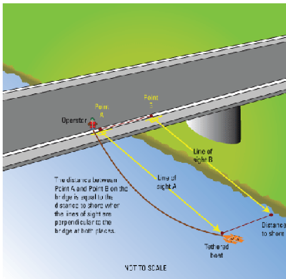
Figure 10. Measuring edge distances when using a tethered
