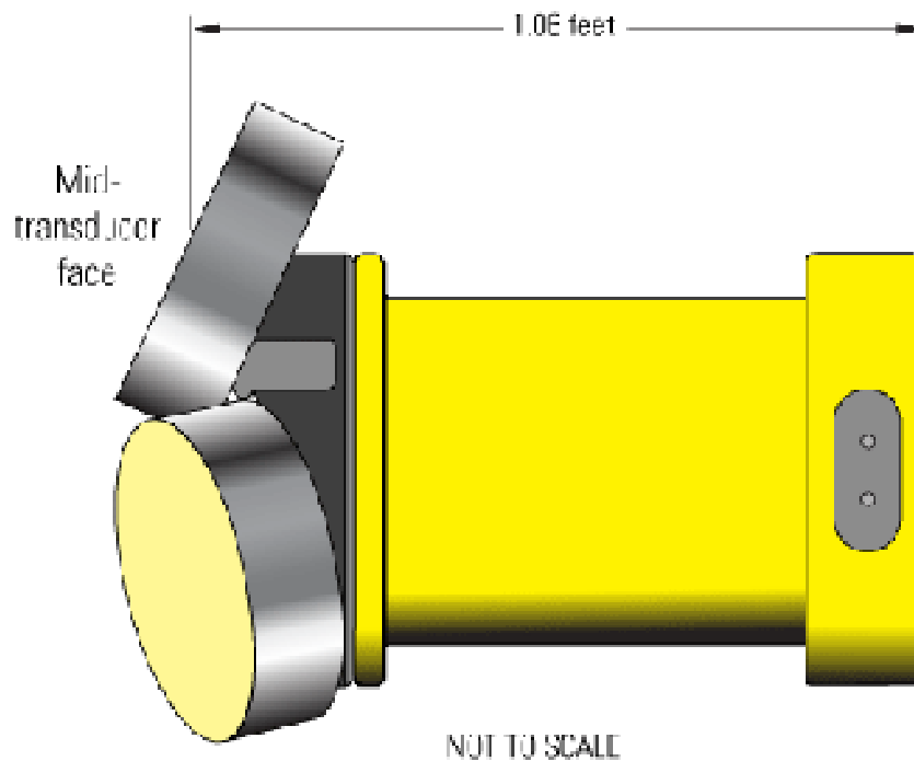
Figure B-2. Distance between top cap and center of transducers for SonTek/YSI 500 kHz acoustic Doppler profiler (ADP).
