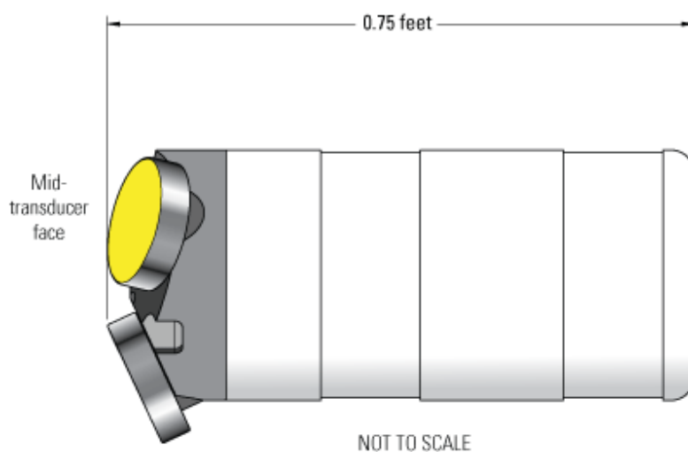
Figure B-3. Distance between top cap and center of transducers for SonTek/YSI 1,500 kHz mini acoustic Doppler profilers (ADPs) with small transducers.
