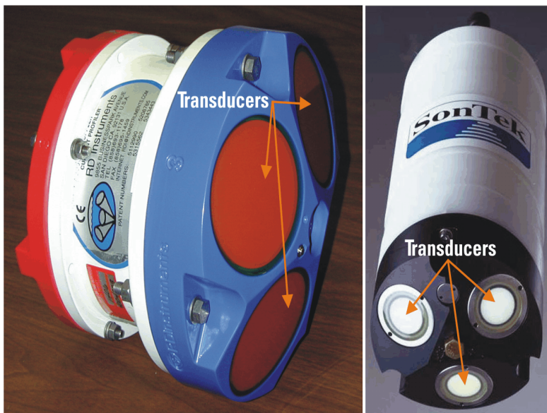
Figure 1. Two acoustic Doppler current profilers commonly used by the U.S. Geological Survey to measure streamflow. (Left photograph by Kevin Oberg, U.S. Geological Survey and right photograph by SonTek/YSI.)
