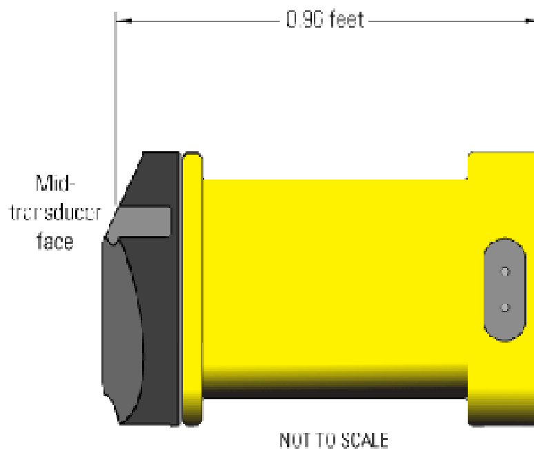
Figure B-1. Distance between top cap and center of transducers for SonTek/YSI 1,000, 1,500, 3,000 kilohertz (kHz) acoustic Doppler profilers (ADPs).
