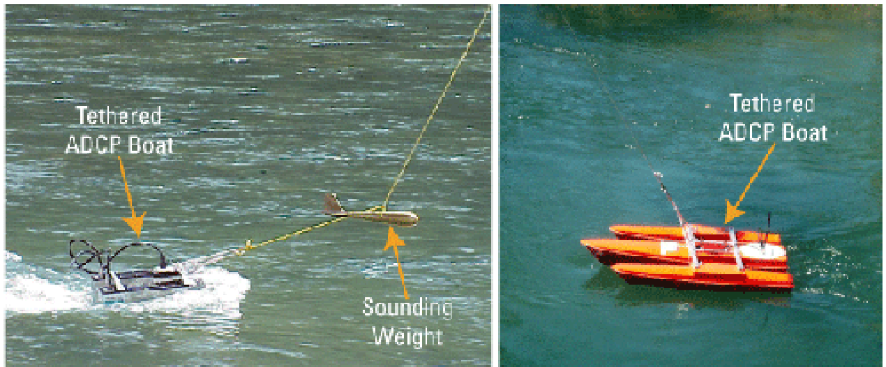
Figure 5. Examples of tethered acoustic Doppler current profiler (ADCP) boats used for making discharge measurements. (Left photograph by Jeff Woodward, Environment Canada and right photograph by Geoffrey D. Cartano, U.S. Geological Survey.)
