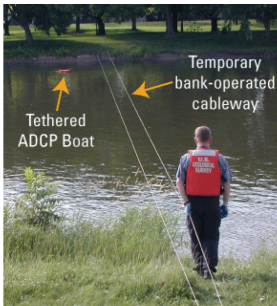
Figure 6. A temporary bank-operated cableway for making acoustic Doppler current profiler (ADCP) measurements with a tethered ADCP boat. (Photograph by Brian Loving, U.S. Geological Survey.)
